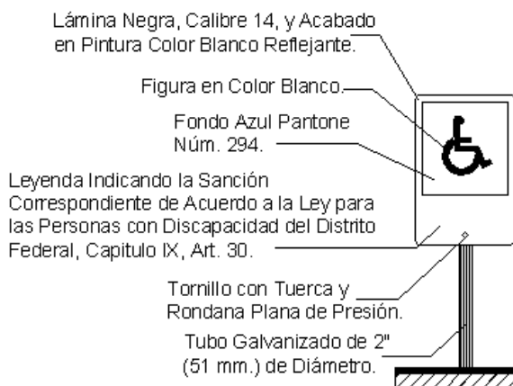
VISTA FRONTAL
